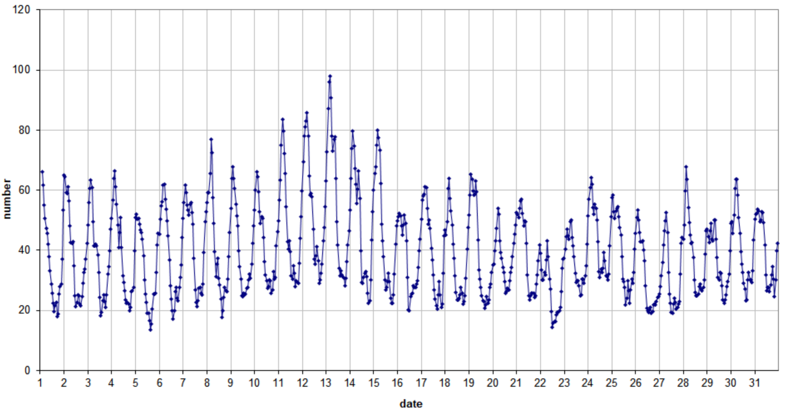
49.99 MHz - RadioMeteors August 2024 number of "all" reflections per hour (weighted average) (automatic count_Mettel5_7Hz) Felix Verbelen (Kamphenhout)
