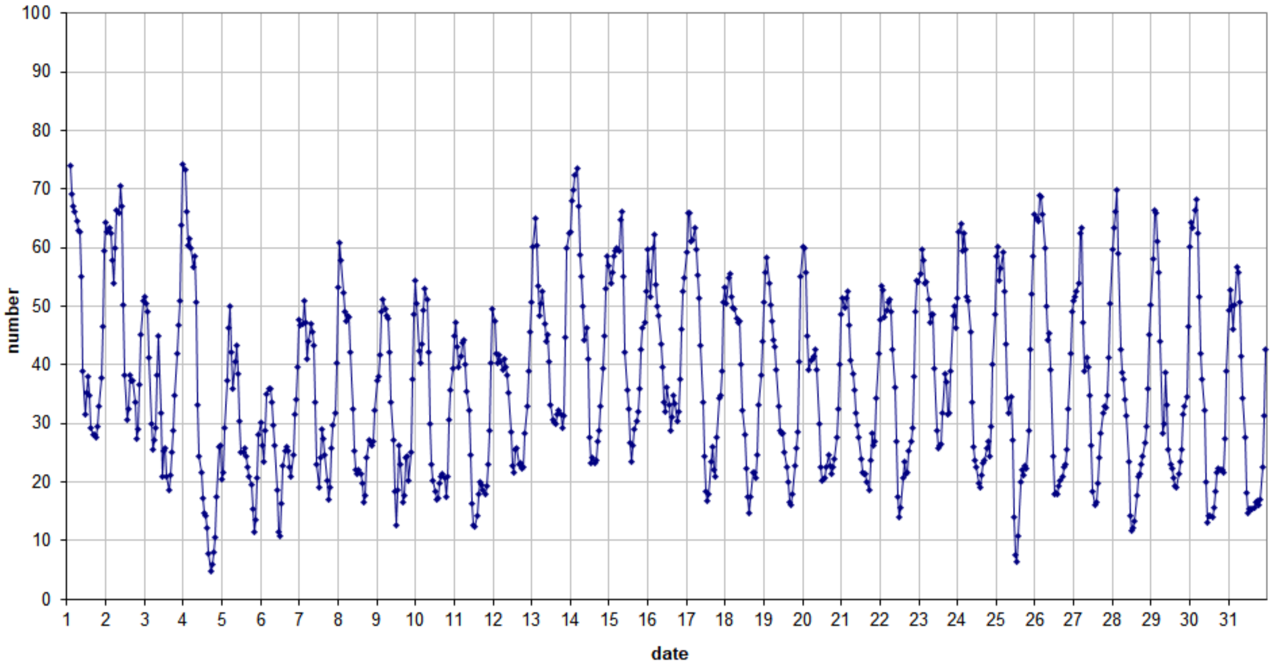
49.99 MHz - RadioMeteors July 2024 number of "all" reflections per hour (weighted average) (automatic count_Mettel5_7Hz) Felix Verbelen (Kampenhout)
