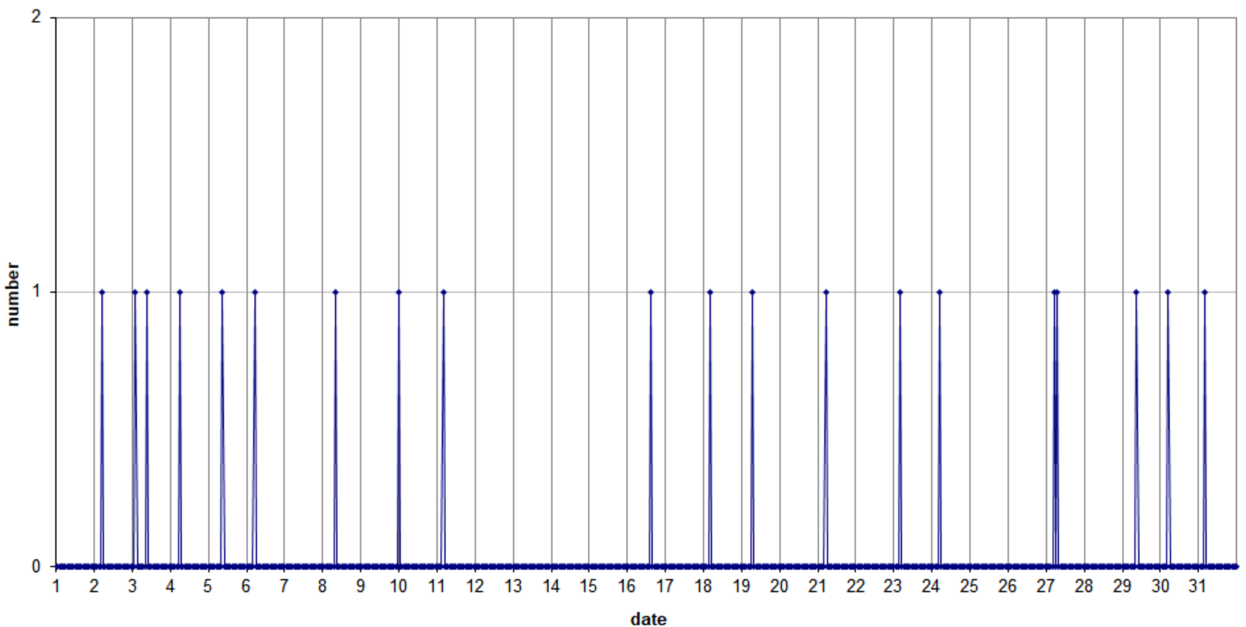
49.99MHz - RadioMeteors July 2024 hourly totals of overdense reflections longer than 1 minute Felix Verbelen (Kampenhout/BE)
