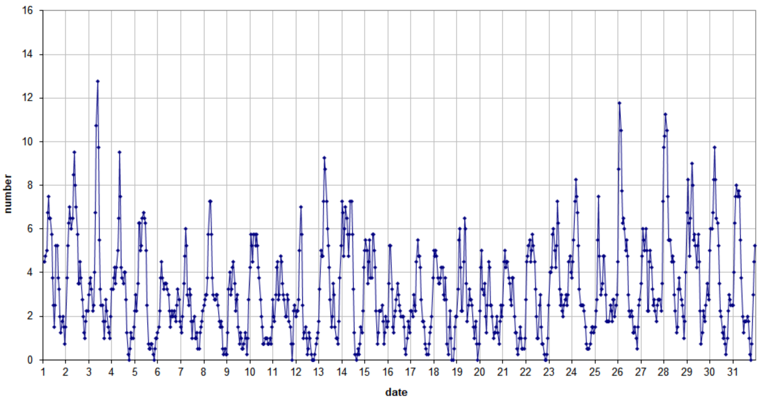
49.99MHz - RadioMeteors July 2024 number of overdense reflections per hour (weighted average) Felix Verbelen (Kampenhout)
