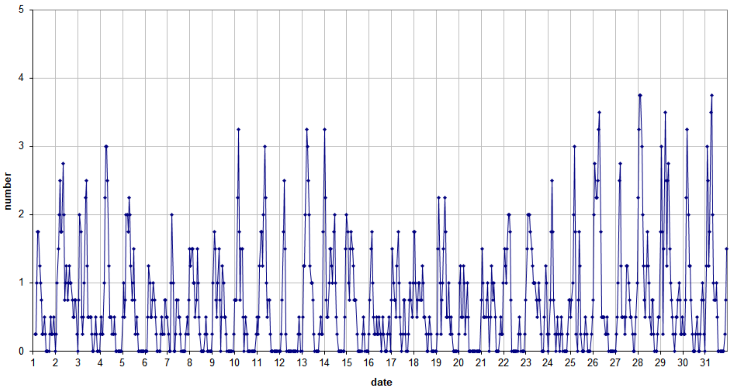
49.99MHz - RadioMeteors July 2024 number of reflections >10 seconds per hour (weighted average) Felix Verbelen (Kampenhout)
