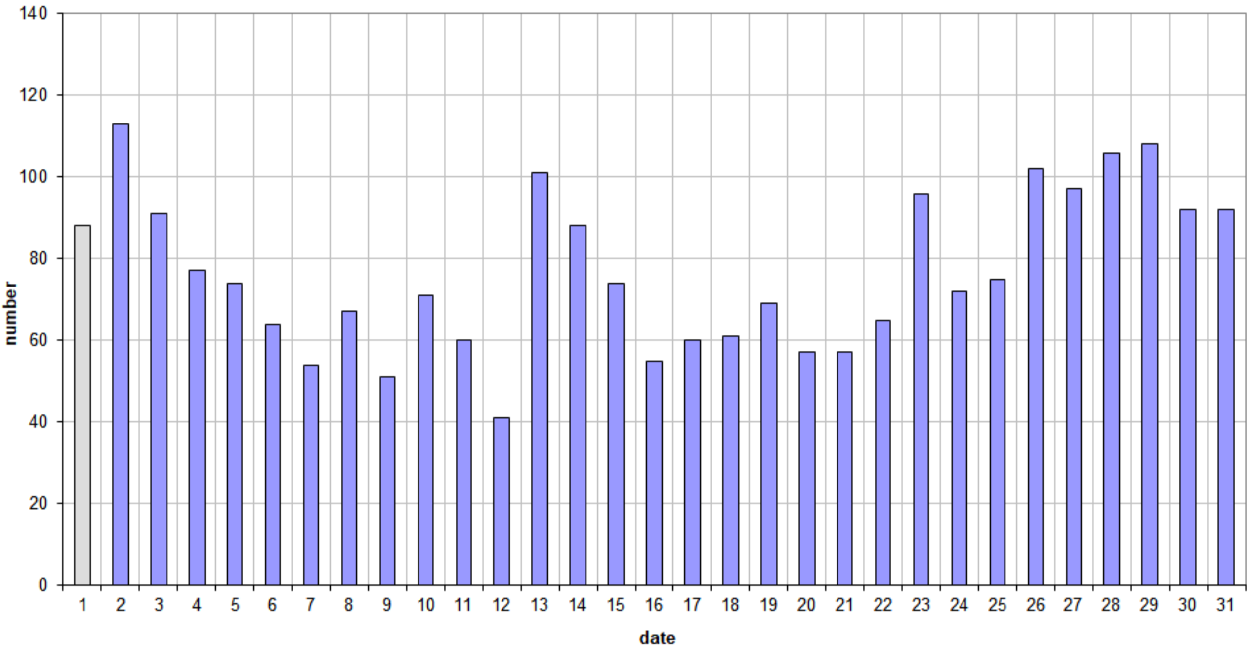
49.99MHz - RadioMeteors July 2024 daily totals of all overdense reflections Felix Verbelen (Kamphenhout)
