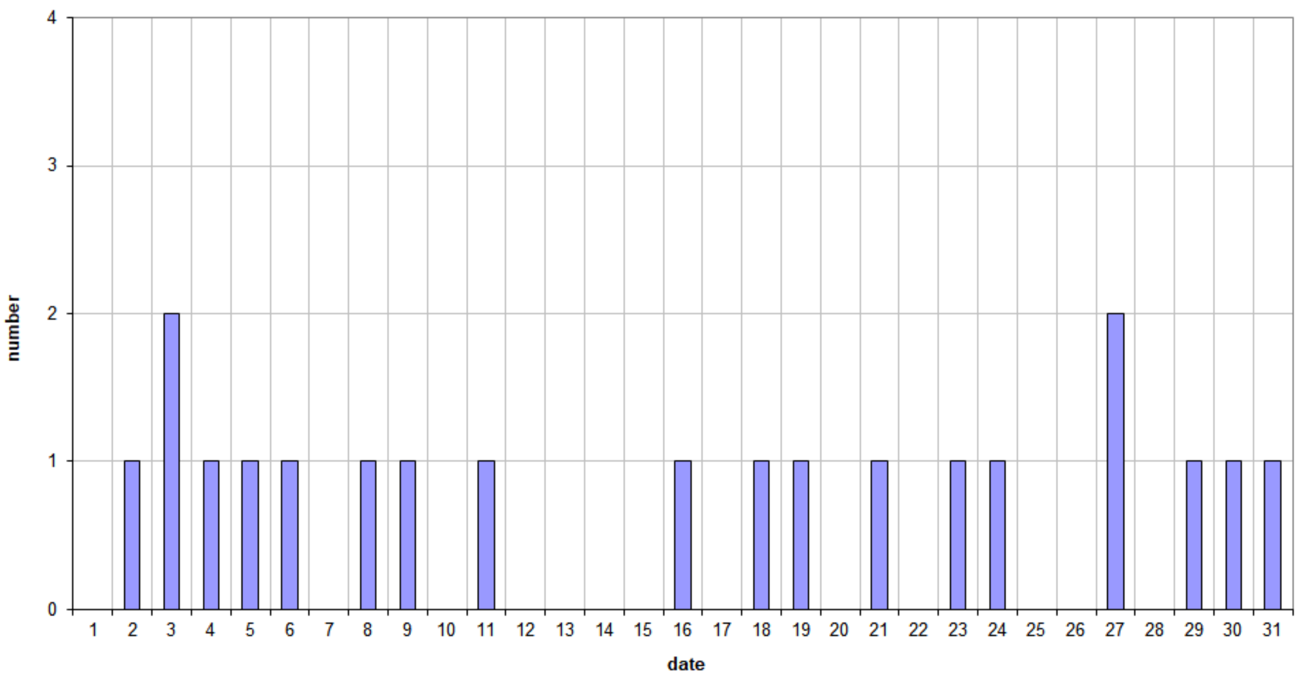
49.99MHz - RadioMeteors July 2024 daily totals of reflections longer than 1 minute Felix Verbelen (Kamphenhout)
