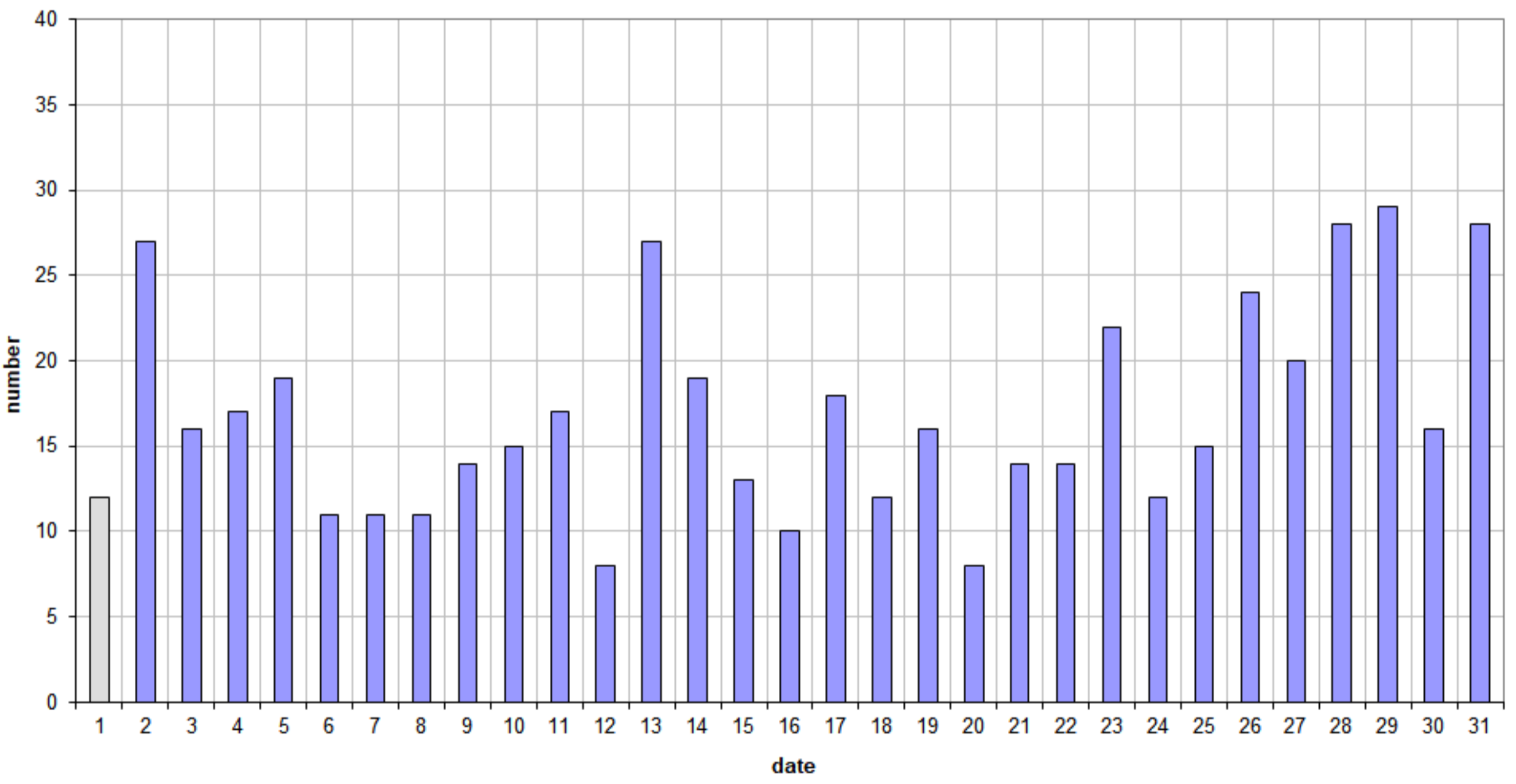
49.99MHz - RadioMeteors July 2024 daily totals of reflections longer than 10 seconds Felix Verbelen (Kamphenhout)
