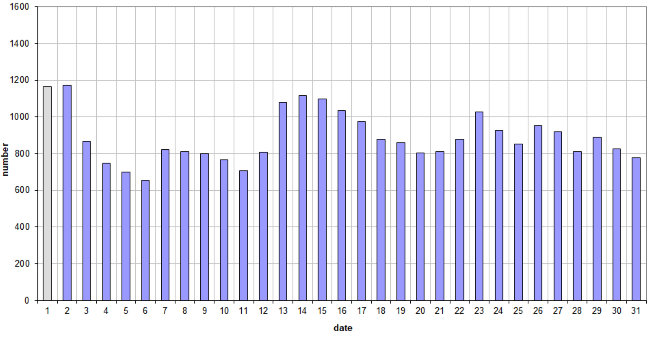
49.99MHz - RadioMeteors July 2024 daily totals of "all" reflections (automatic count_Mettel5_7Hz) Felix Verbelen (Kamphenhout)
