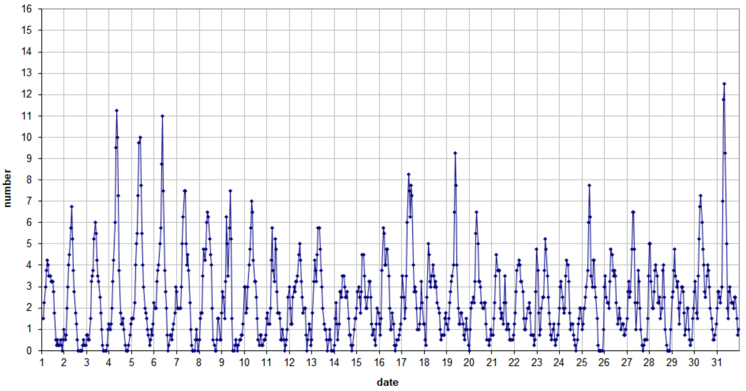
49.99MHz - RadioMeteors May 2024 number of overdense reflections per hour (weighted average) Felix Verbelen (Kampenhout)
