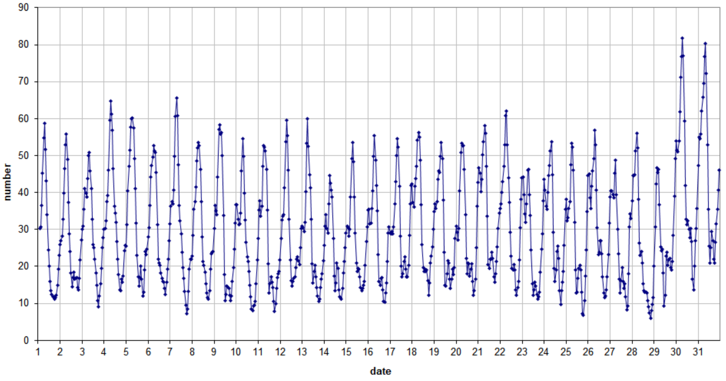
49.99 MHz - RadioMeteors May 2024 number of "all" reflections per hour (weighted average) (automatic count_Mettel5_7Hz) Felix Verbelen (Kampenhout)
