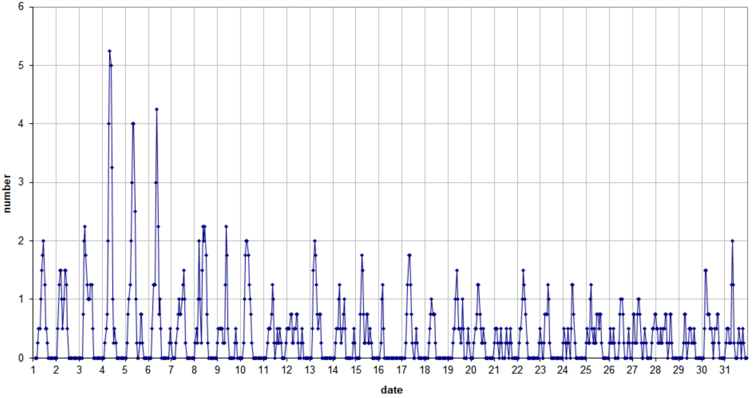
49.99MHz - RadioMeteors May 2024 number of reflections >10 seconds per hour (weighted average) Felix Verbelen (Kampenhout)
