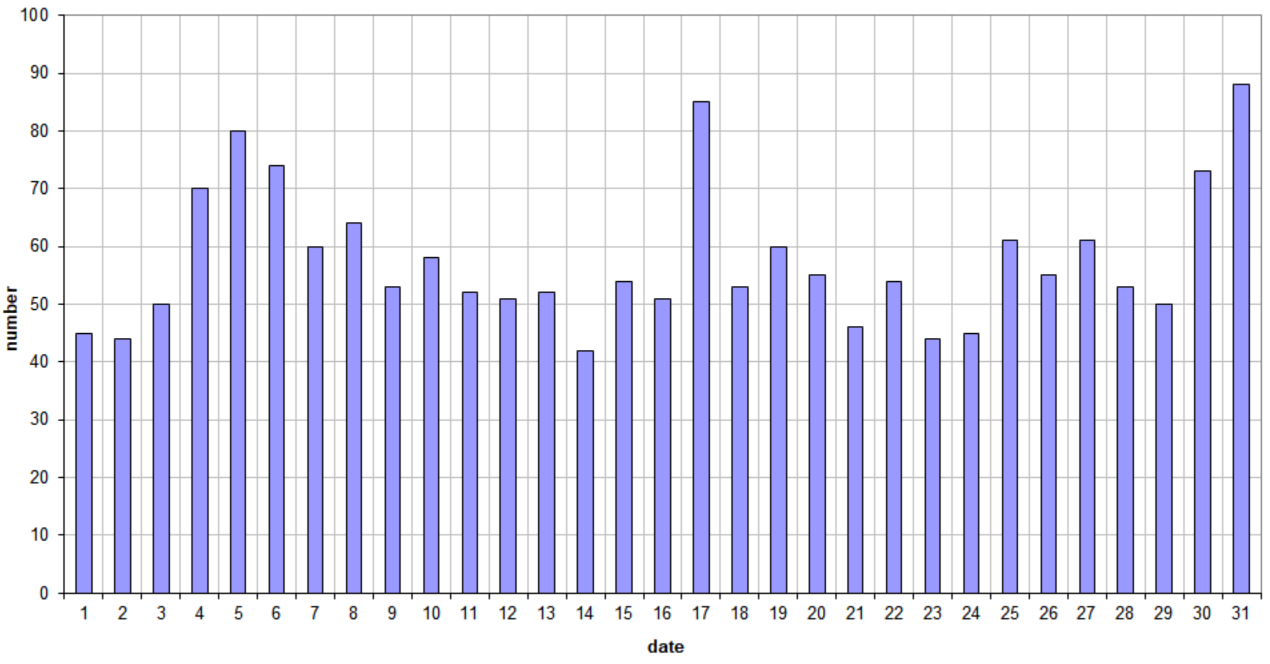
49.99MHz - RadioMeteors May 2024 daily totals of all overdense reflections Felix Verbelen (Kamphenhout)
