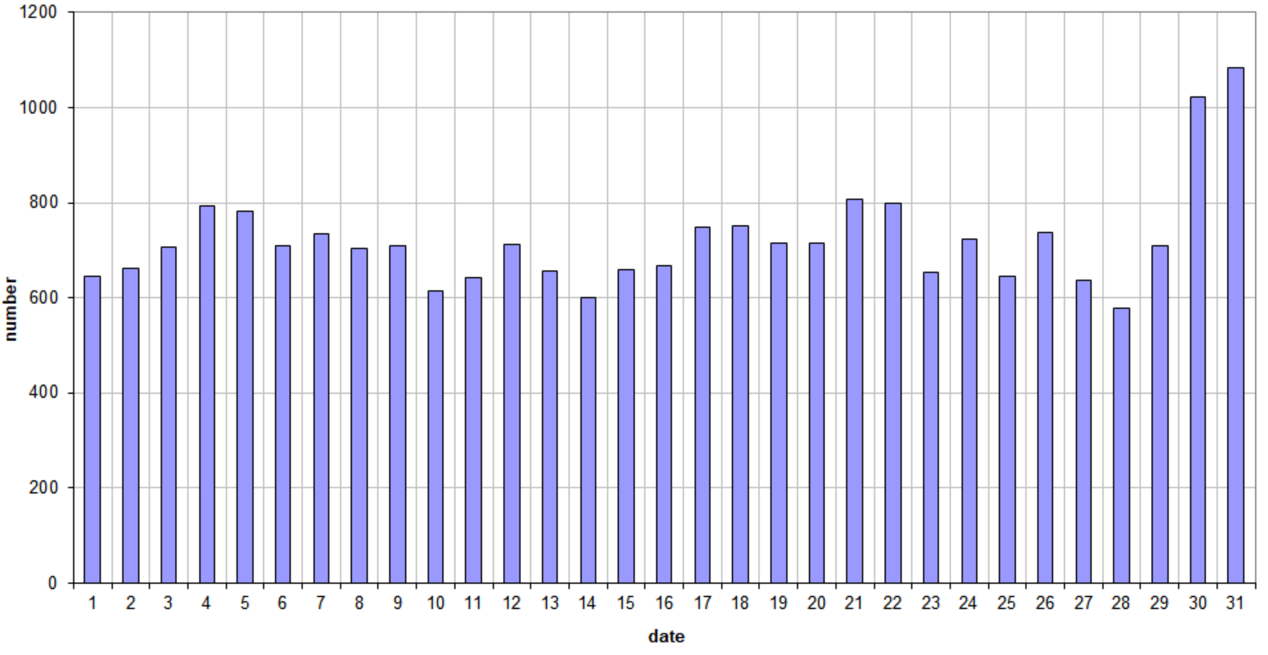
49.99MHz - RadioMeteors May 2024 daily totals of "all" reflections (automatic count_Mettel5_7Hz) Felix Verbelen (Kamphenhout)
